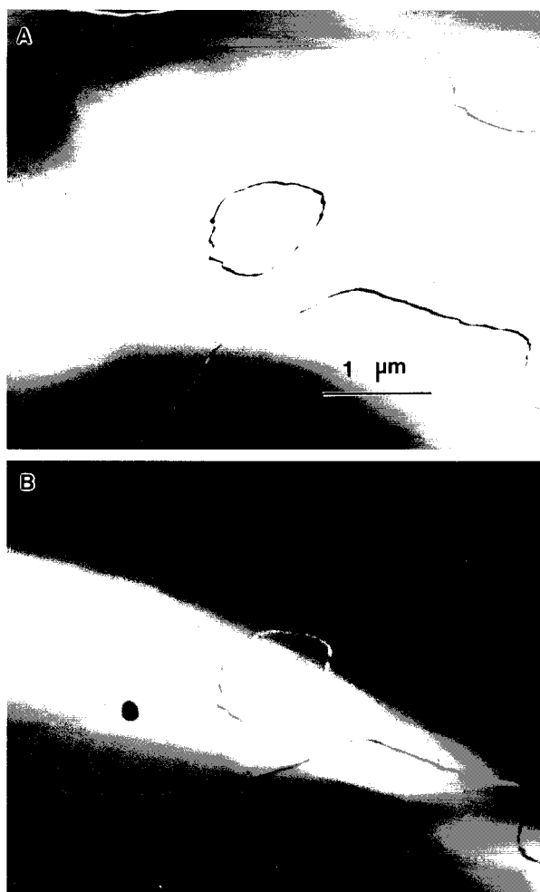
FIGURE 9. Dark-field images of c-APBs. (A) Original configuration; (B) after the specimen was cycled successively about T_c for 10 min, with \Delta T_0 = 100, 200, 300, 400, 500, 600, and 700 °C.
