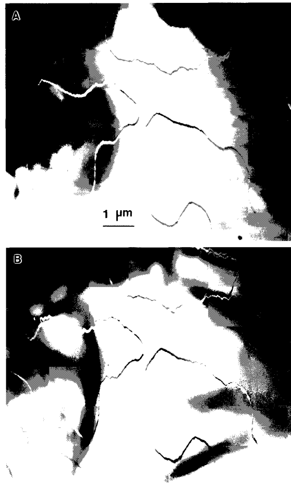
FIGURE 8. Dark-field images of c-APBs. (A) Original configuration; (B) after the specimen was cycled successively about T_c , with \Delta T_c = 350 °C for 1, 10, 20, 50, 100, 200, 500, 1000, and 2000 s.
