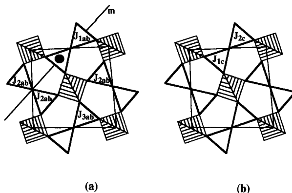
FIGURE 7. Definition of the interactions, J , between the T2 sites marked by the heavy dot and other T2 tetrahedra as marked: (a) in the a - b plane, (b) in the next layer in the \pm c direction. Note the mirror plane m .
