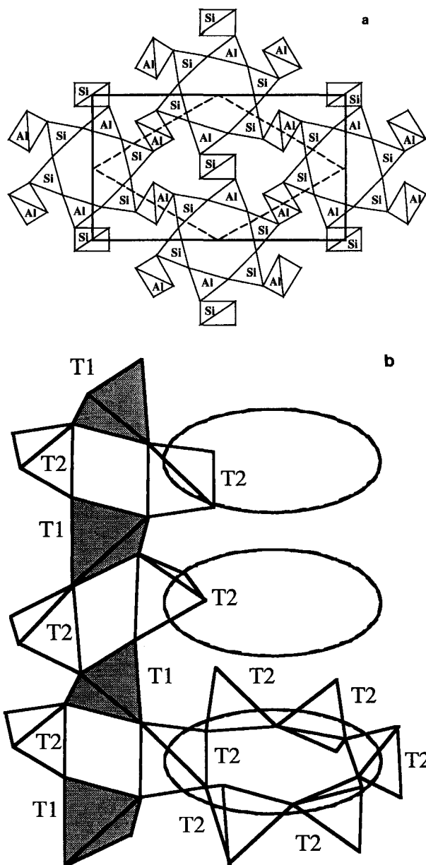
FIGURE 11. The cordierite structure. (a) Hexagons of T2 sites in an a-b plane are linked by T1 sites lying half-way between successive planes of T2 sites. The ordering and orthorhombic unit cell are shown. (b) A chain of square rings parallel to the c axis consist of T1 sites linking adjacent hexagons of T2 sites in one a-b layer and hexagons in adjacent layers.
