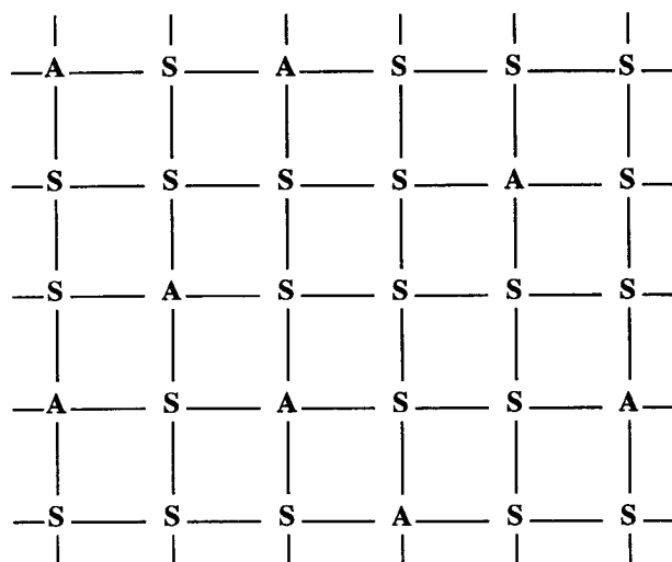
FIGURE 8. One of many arrangements of Al (A) and Si (S) atoms on a planar square lattice with the proportion of Al atoms x = 0.25 , in which each Al atom has 4 Si nearest neighbors, showing no long-range order. Each such configuration has no Al-Al linkages and has the same energy ignoring all interactions beyond nearest-neighbors.
